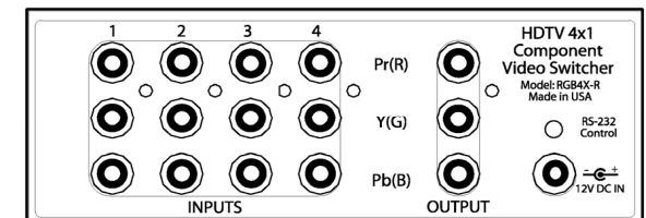
Figure 1 -Connectors
