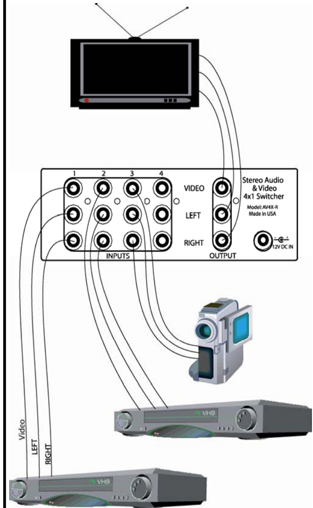
Figure 2 - Typical Setup
