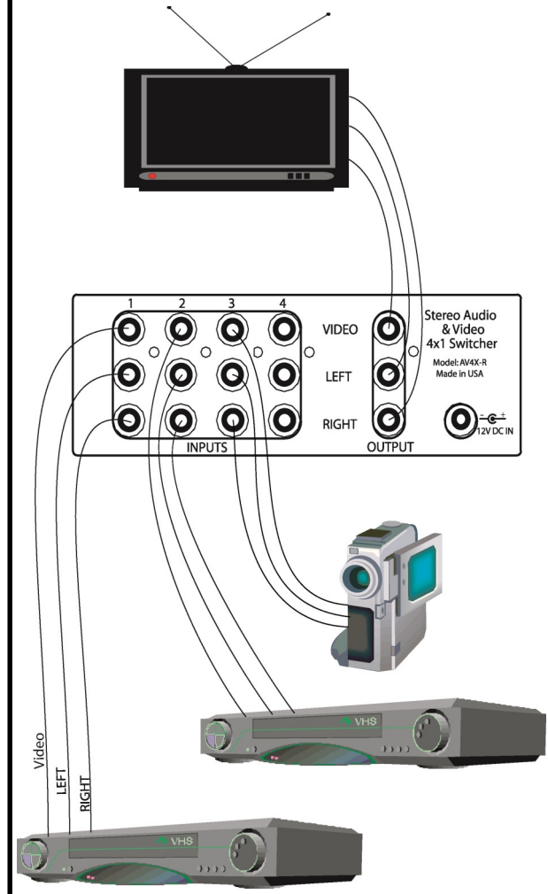
Figure 2 - Typical Setup
